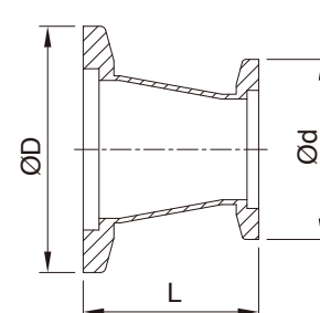
Conical Reducer
