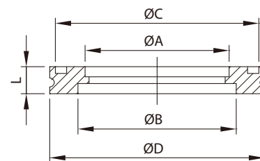
Weld Flange
