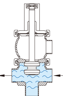
Open
