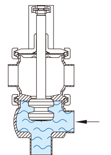
Open
